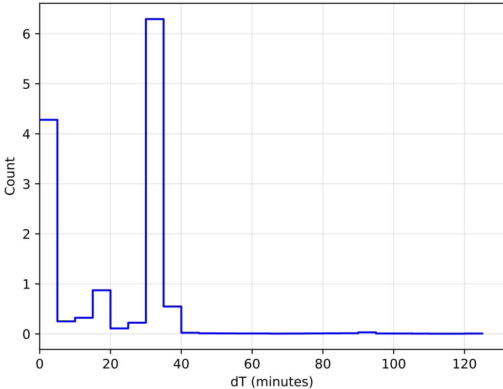
too_elab_r16_d2_griz_v3.4_10yrs All sky: DeltaT Histogram 1e6
