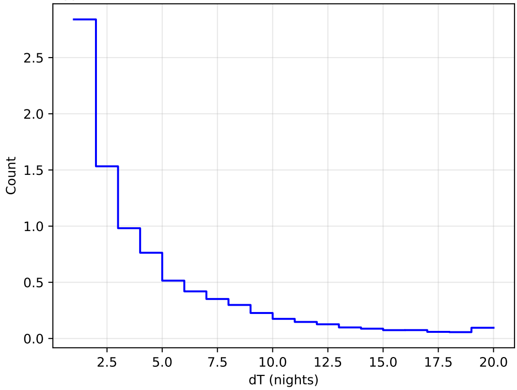
too_elab_r16_d2_griz_v3.4_10yrs All sky all bands: DeltaNight Histogram
