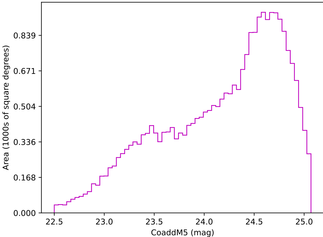
too_elab_r16_d2_griz_v3.4_10yrs Yr 3-4 z band: CoaddM5
