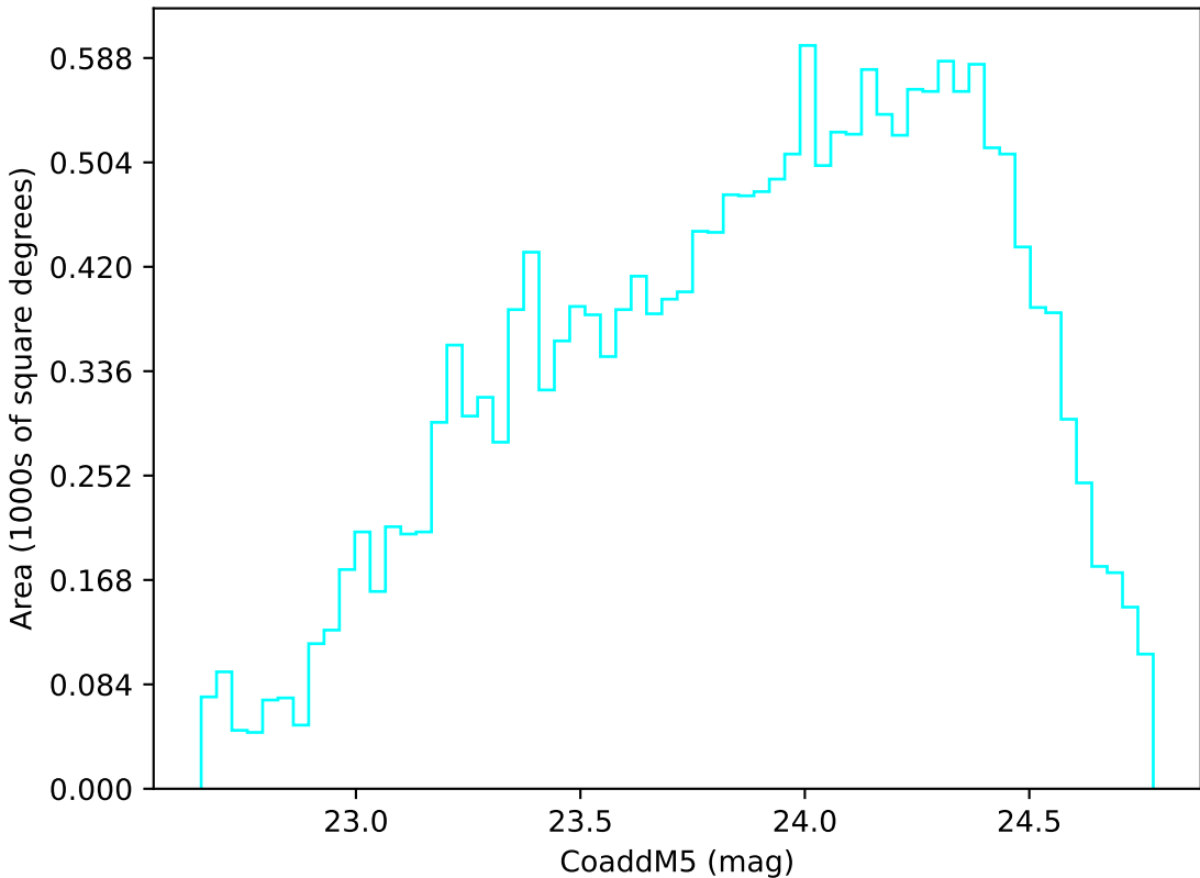
too_elab_r16_d2_griz_v3.4_10yrs Yr 3-4 u band: CoaddM5
