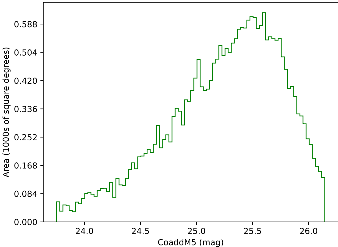
too_elab_r16_d2_griz_v3.4_10yrs Yr 3-4 g band: CoaddM5
