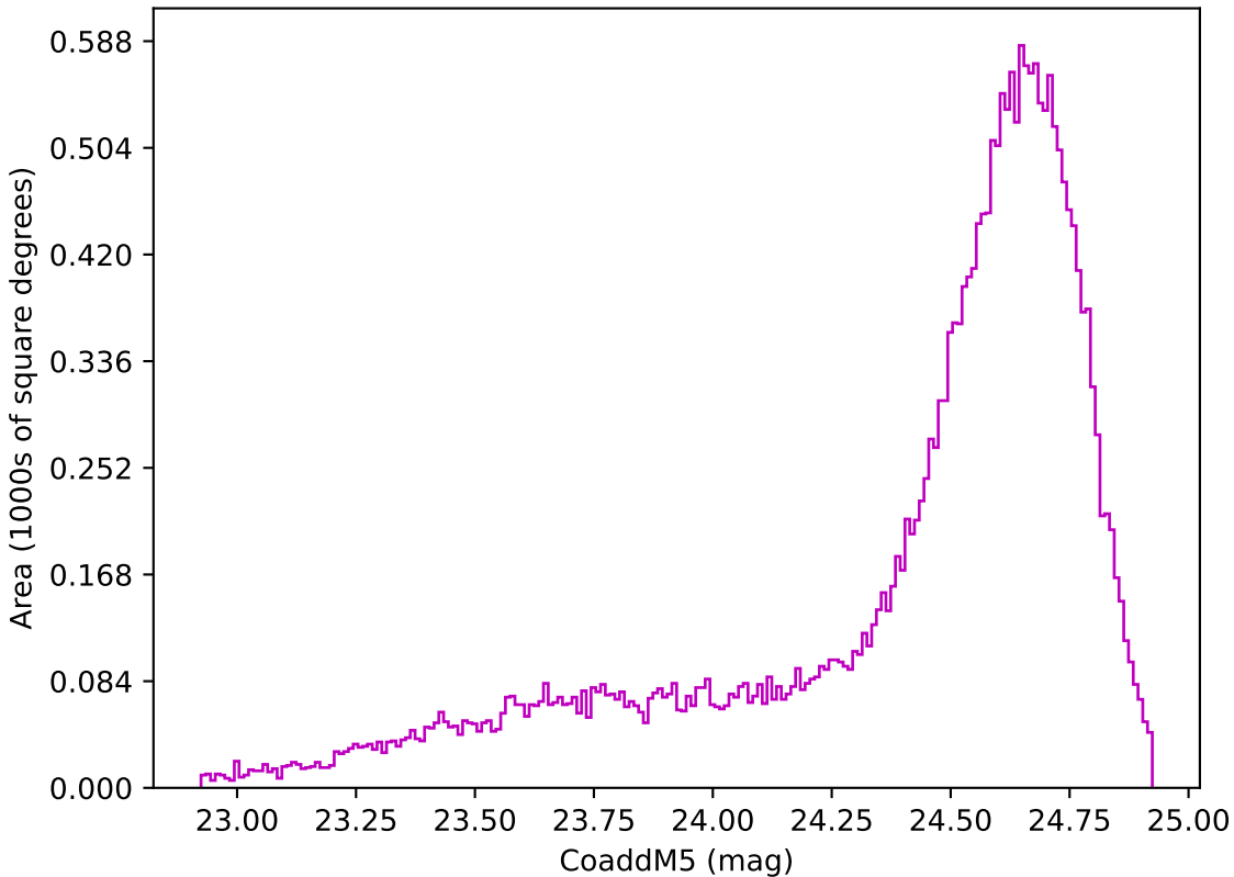
too_elab_r16_d2_griz_v3.4_10yrs Yr 1 z band: CoaddM5
