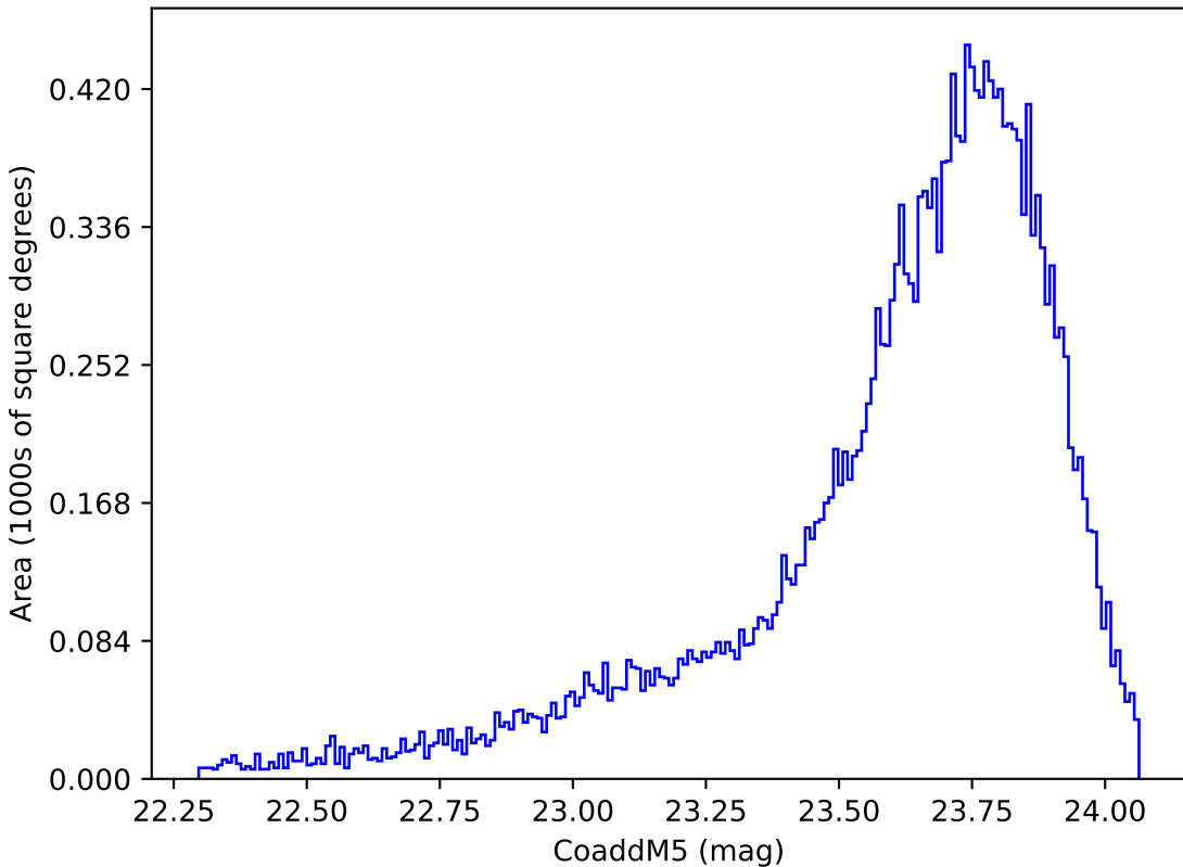
too_elab_r16_d2_griz_v3.4_10yrs Yr 1 y band: CoaddM5
