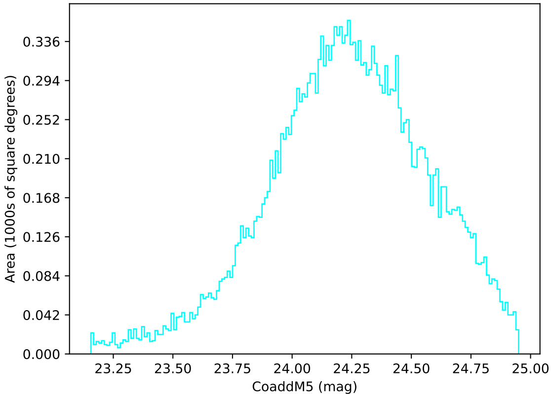
too_elab_r16_d2_griz_v3.4_10yrs Yr 1 u band: CoaddM5
