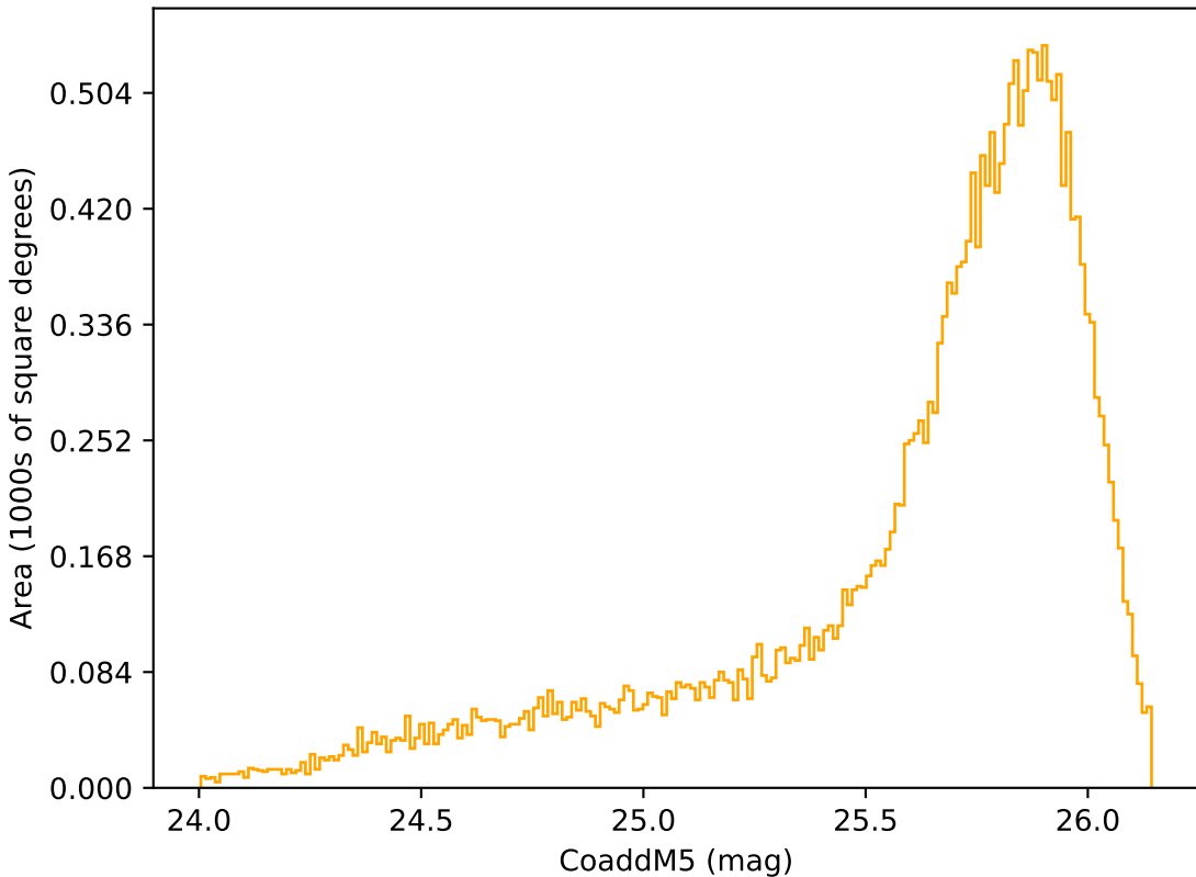
too_elab_r16_d2_griz_v3.4_10yrs Yr 1 r band: CoaddM5
