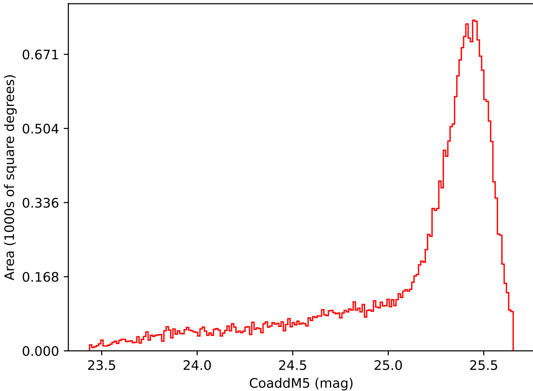
too_elab_r16_d2_griz_v3.4_10yrs Yr 1 i band: CoaddM5
