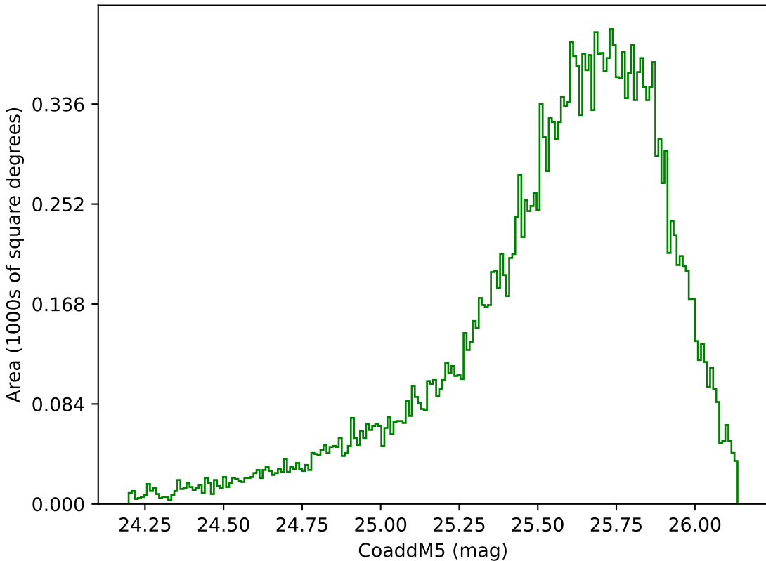
too_elab_r16_d2_griz_v3.4_10yrs Yr 1 g band: CoaddM5
