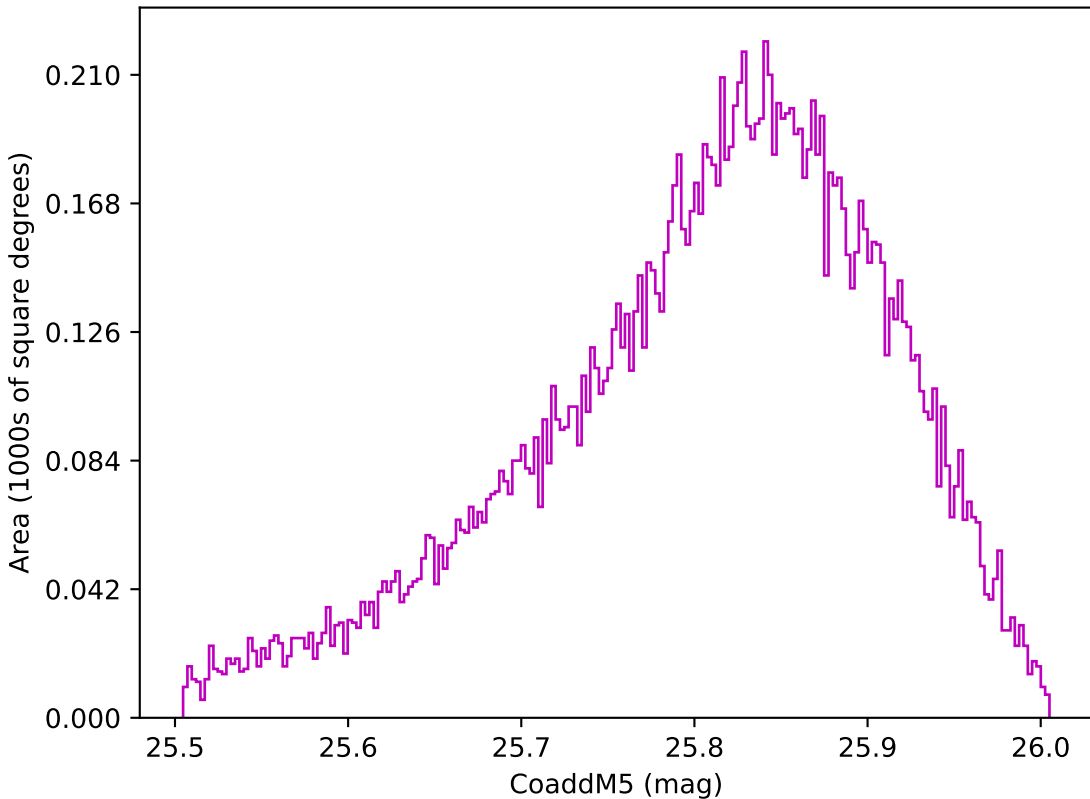
too_elab_r16_d2_griz_v3.4_10yrs WFD z band: CoaddM5
