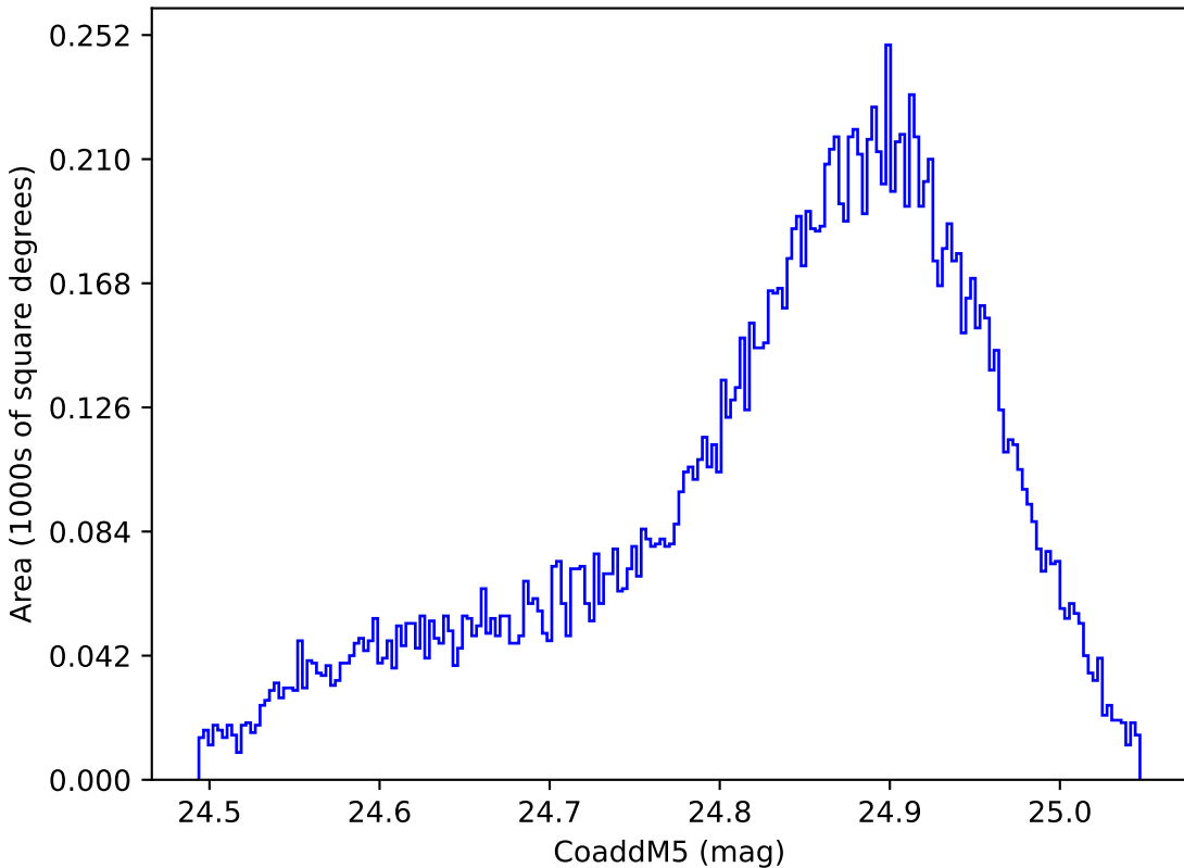
too_elab_r16_d2_griz_v3.4_10yrs WFD y band: CoaddM5
