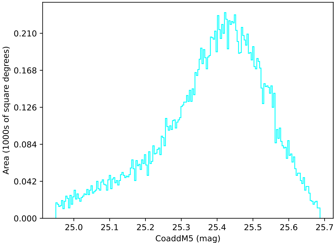
too_elab_r16_d2_griz_v3.4_10yrs WFD u band: CoaddM5
