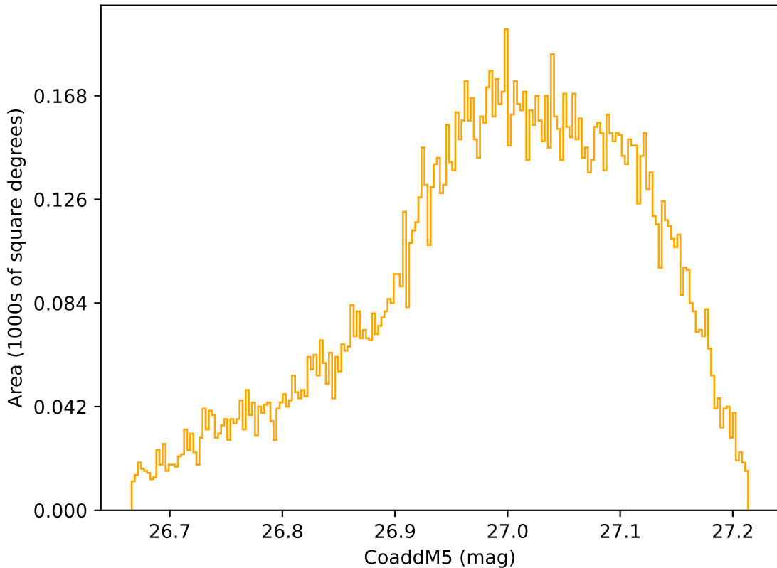
too_elab_r16_d2_griz_v3.4_10yrs WFD r band: CoaddM5
