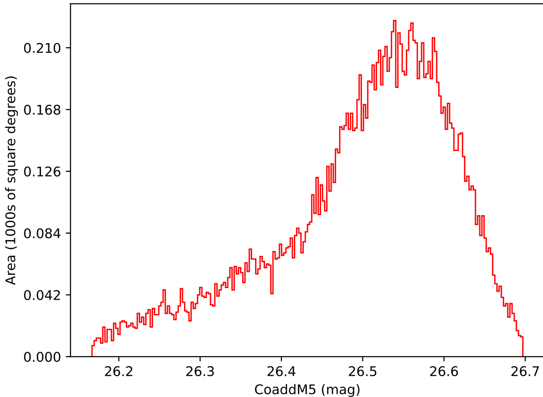
too_elab_r16_d2_griz_v3.4_10yrs WFD i band: CoaddM5
