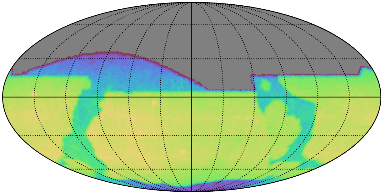
too_elab_r16_d2_griz_v3.4_10yrs All sky z band: CoaddM5
