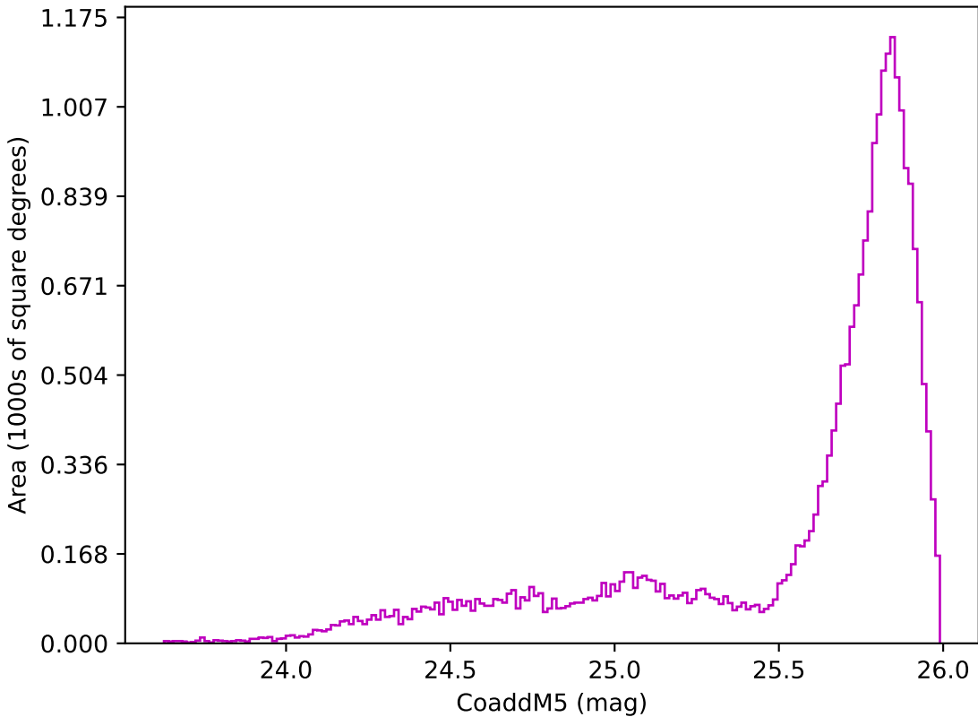
too_elab_r16_d2_griz_v3.4_10yrs All sky z band: CoaddM5
