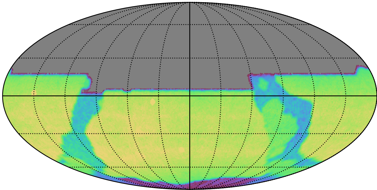
too_elab_r16_d2_griz_v3.4_10yrs All sky y band: CoaddM5
