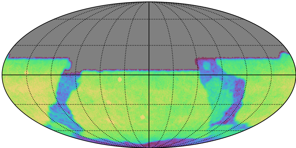
too_elab_r16_d2_griz_v3.4_10yrs All sky u band: CoaddM5
