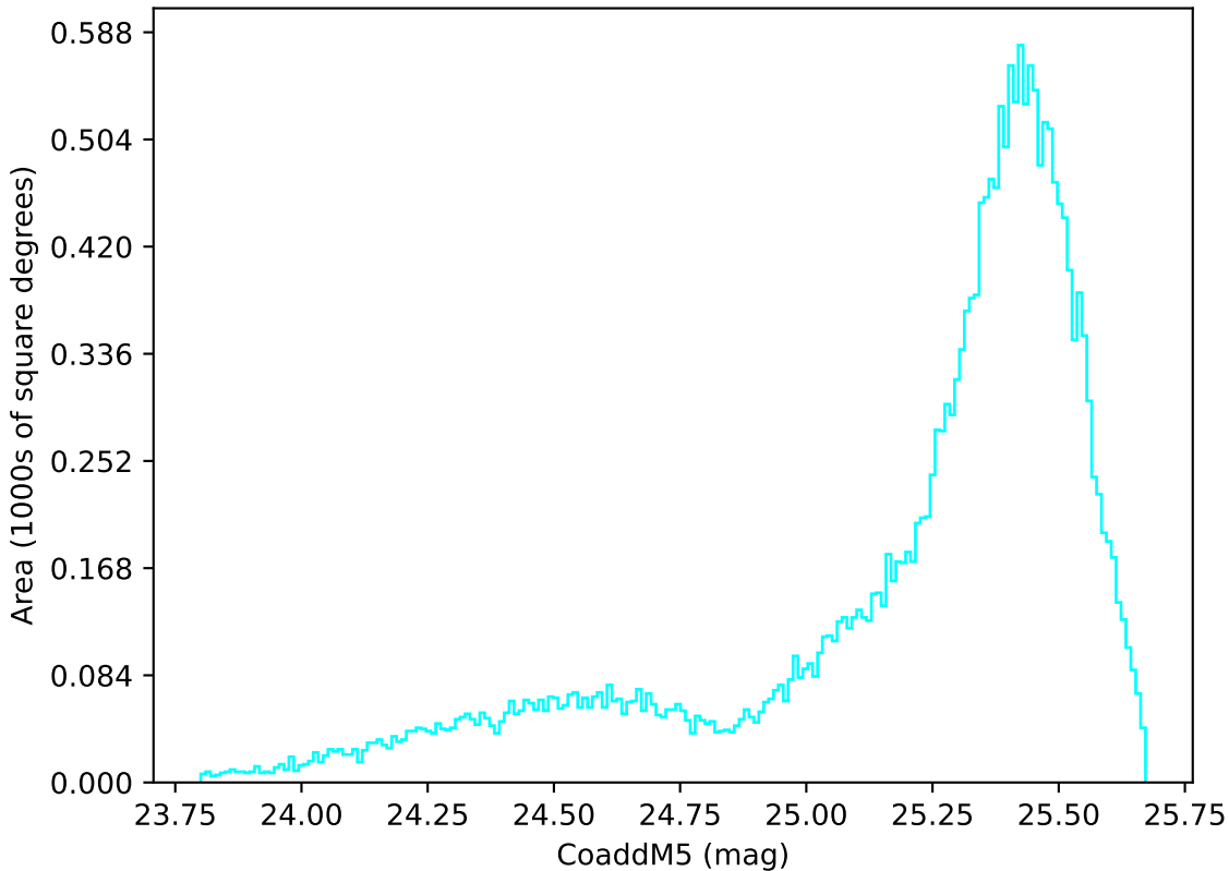
too_elab_r16_d2_griz_v3.4_10yrs All sky u band: CoaddM5
