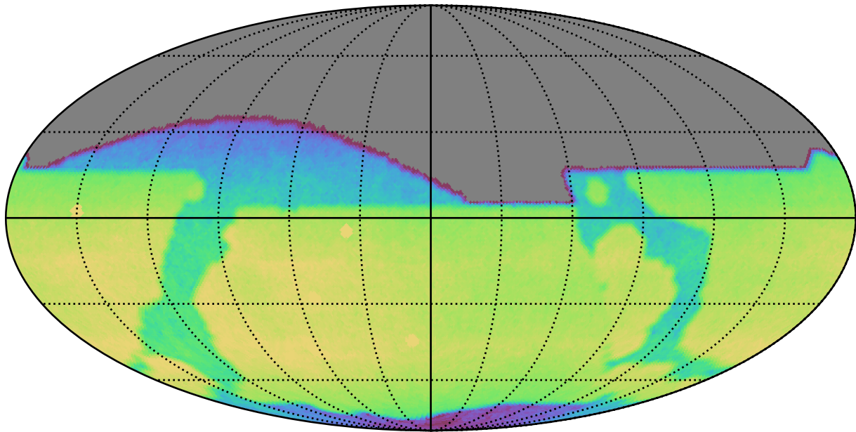
too_elab_r16_d2_griz_v3.4_10yrs All sky r band: CoaddM5
