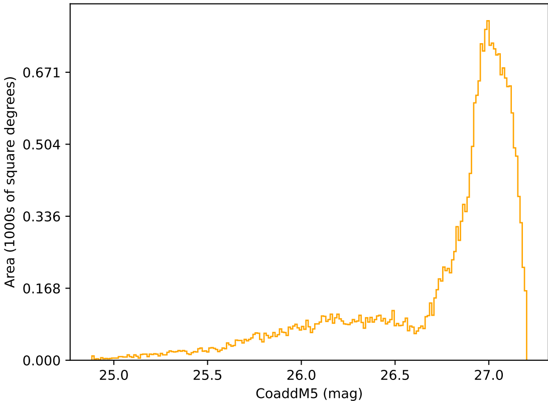
too_elab_r16_d2_griz_v3.4_10yrs All sky r band: CoaddM5
