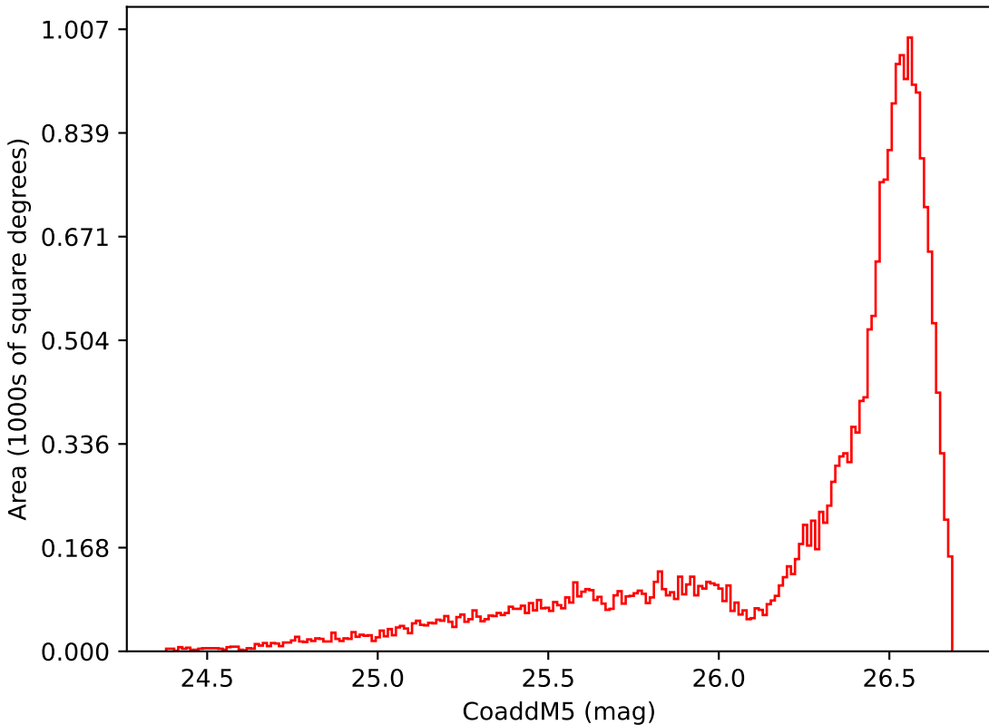
too_elab_r16_d2_griz_v3.4_10yrs All sky i band: CoaddM5
