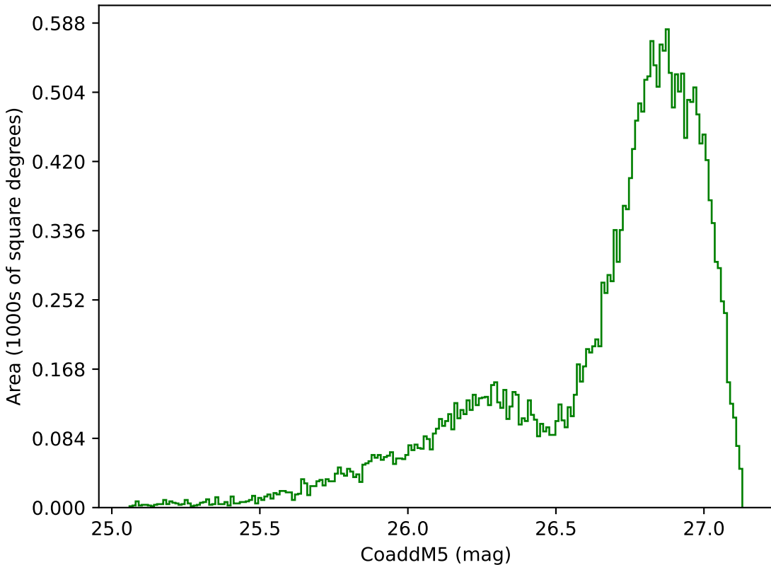
too_elab_r16_d2_griz_v3.4_10yrs All sky g band: CoaddM5
