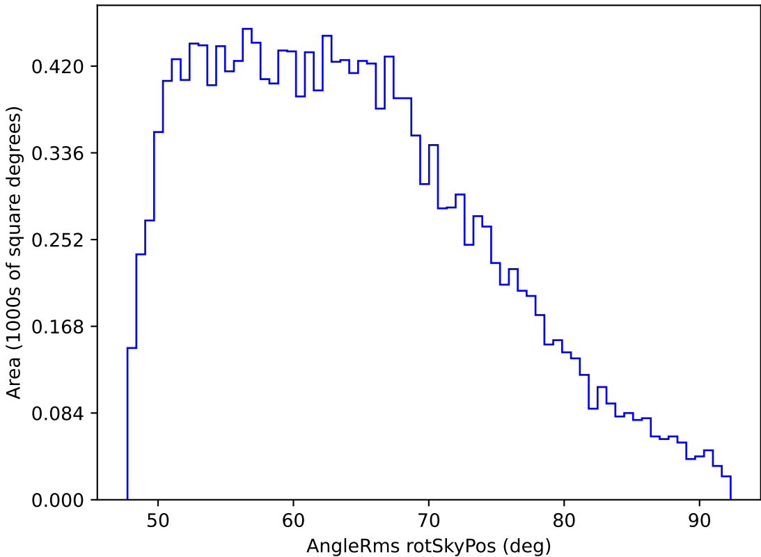
too_elab_r16_d2_griz_v3.4_10yrs WFD i band: AngleRms rotSkyPos
