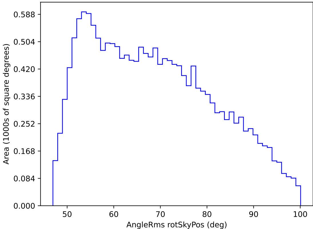
too_elab_r16_d2_griz_v3.4_10yrs WFD g band: AngleRms rotSkyPos
