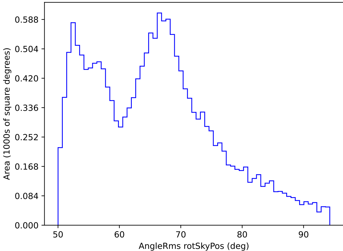
too_elab_r16_d2_griz_v3.4_10yrs WFD all bands: AngleRms rotSkyPos
