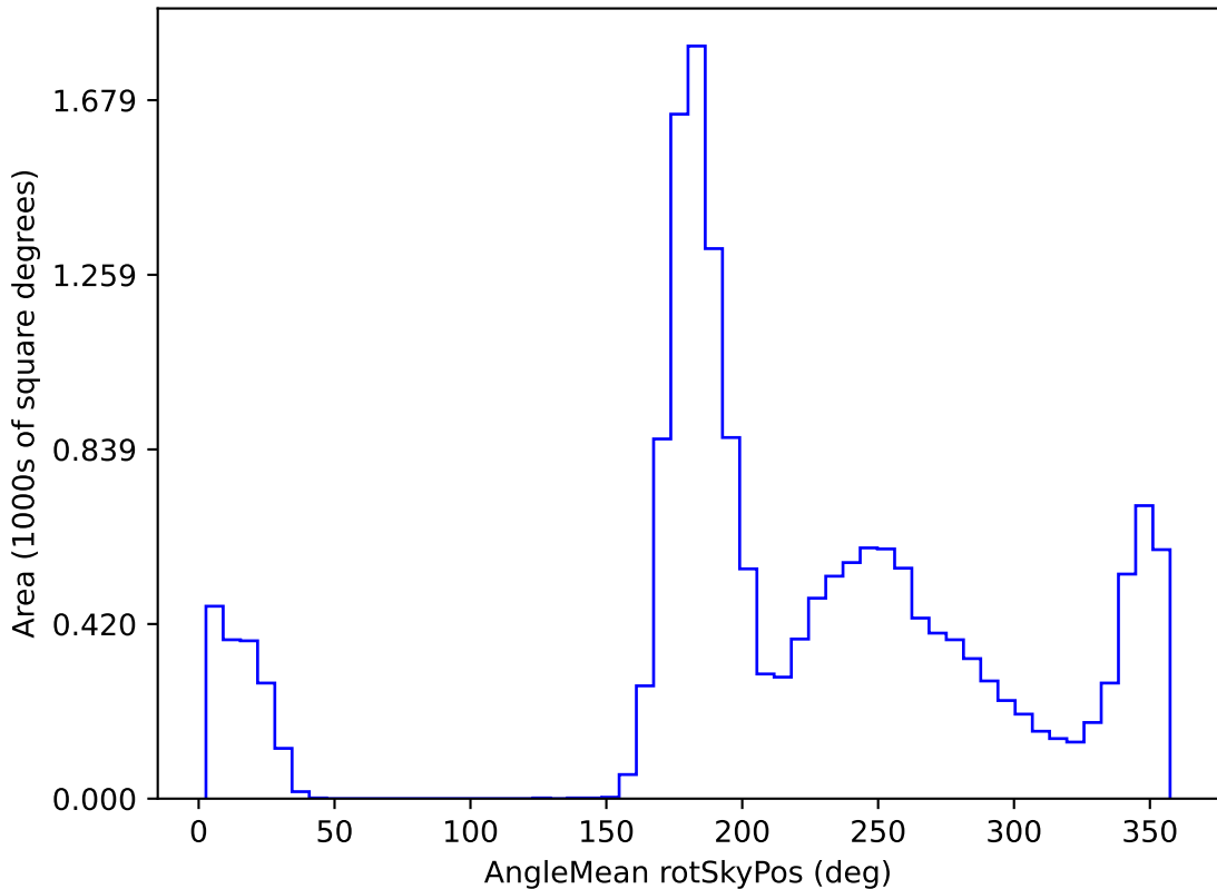
too_elab_r16_d2_griz_v3.4_10yrs WFD i band: AngleMean rotSkyPos
