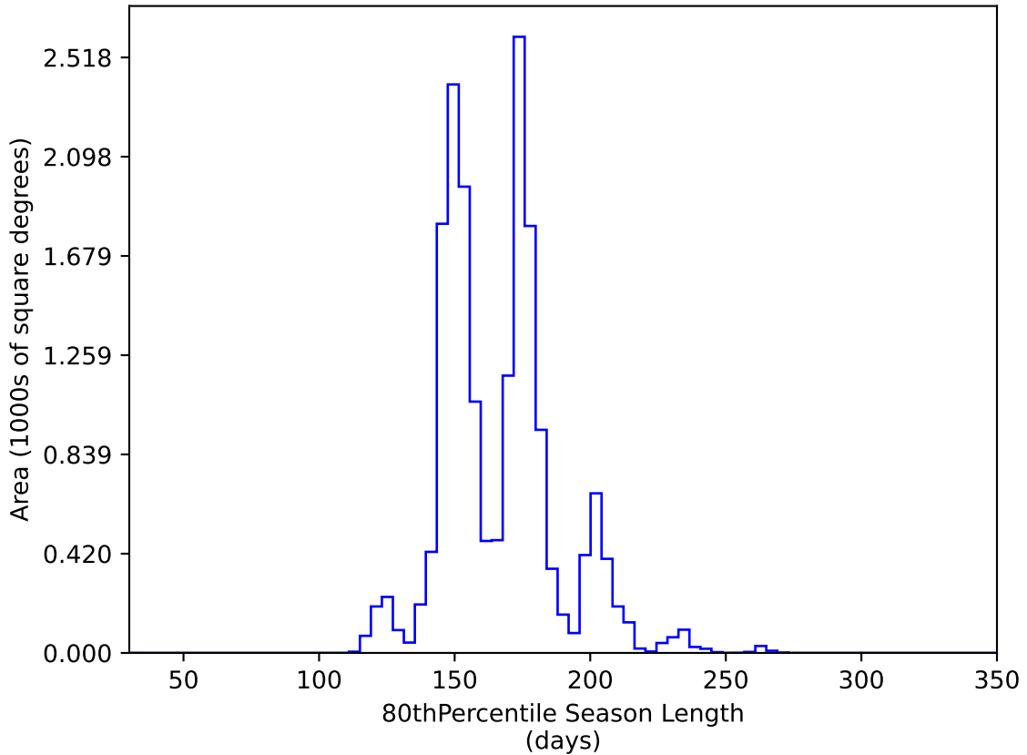
too_elab_r16_d2_griz_v3.4_10yrs WFD y band: 80thPercentile Season Length
