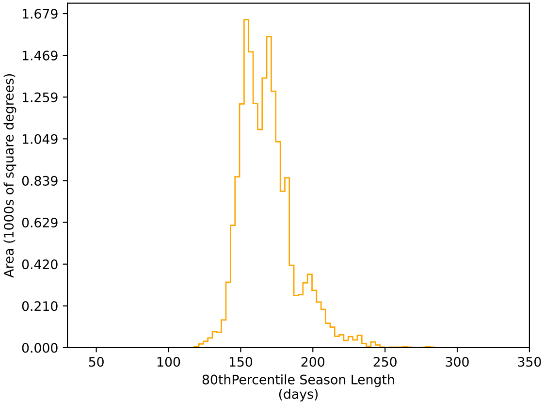
too_elab_r16_d2_griz_v3.4_10yrs WFD r band: 80thPercentile Season Length
