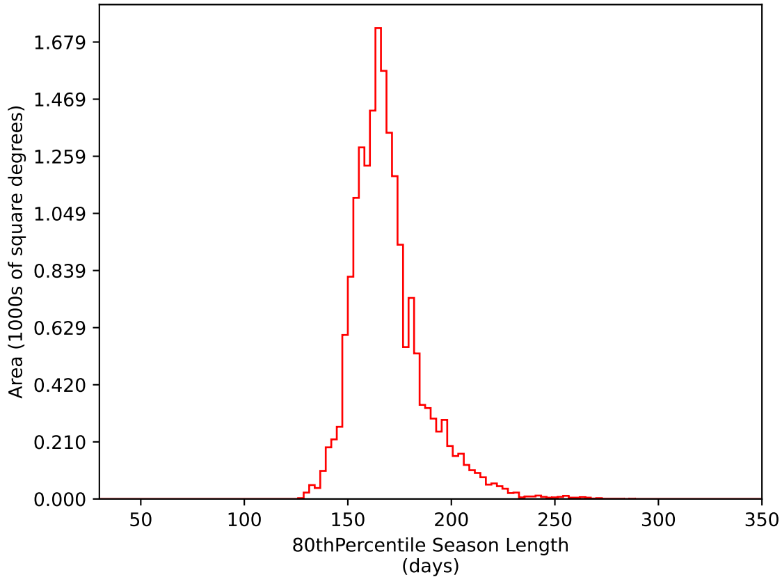
too_elab_r16_d2_griz_v3.4_10yrs WFD i band: 80thPercentile Season Length
