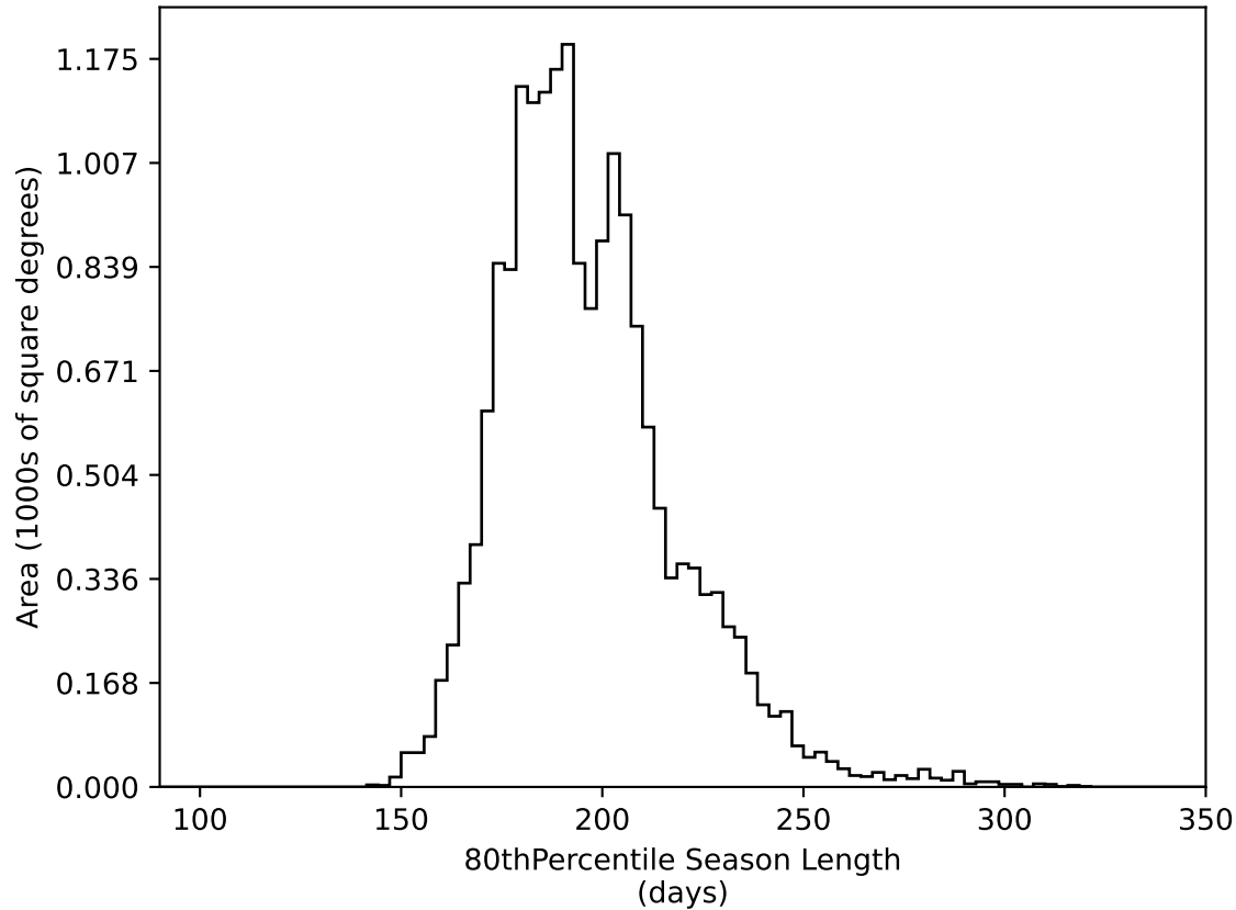
too_elab_r16_d2_griz_v3.4_10yrs WFD all bands: 80thPercentile Season Length
