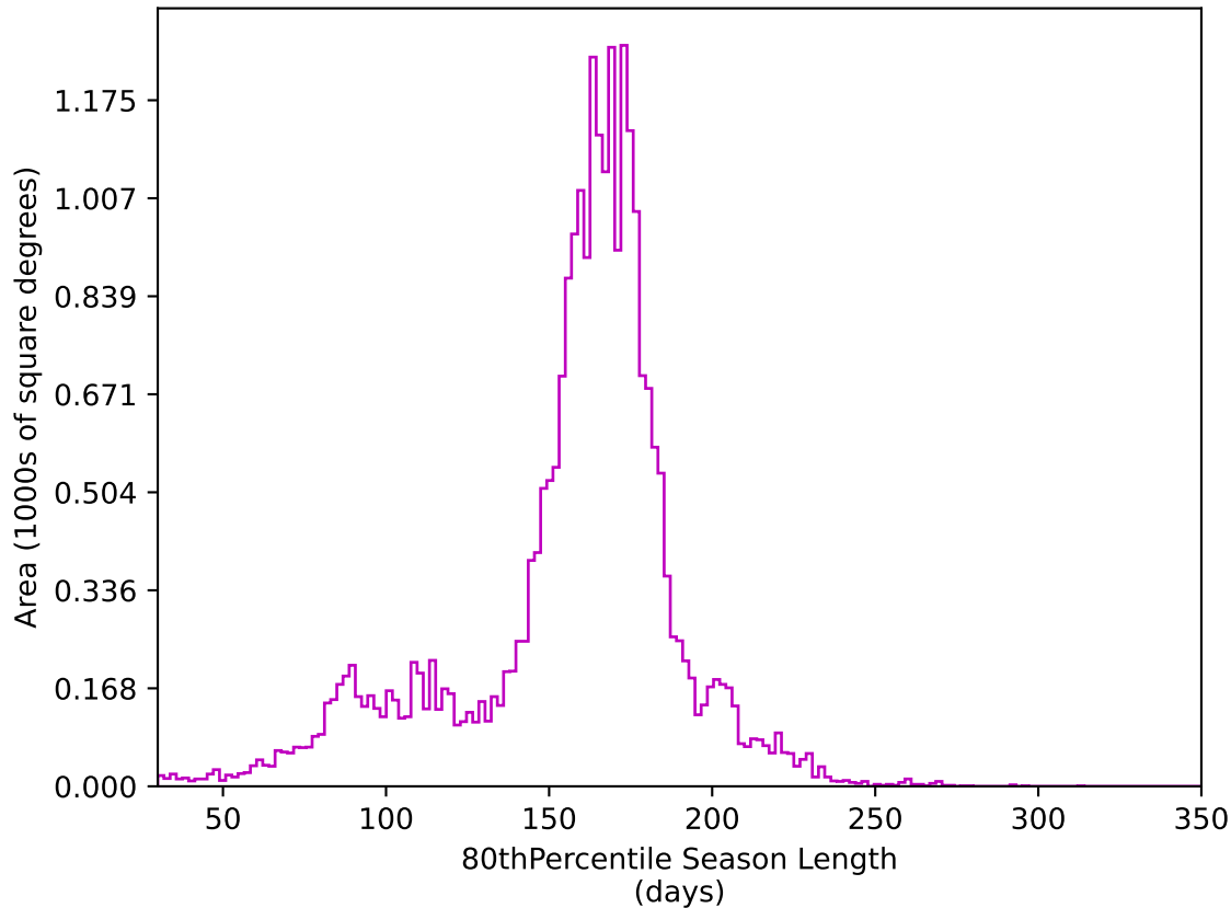
too_elab_r16_d2_griz_v3.4_10yrs All sky z band: 80thPercentile Season Length
