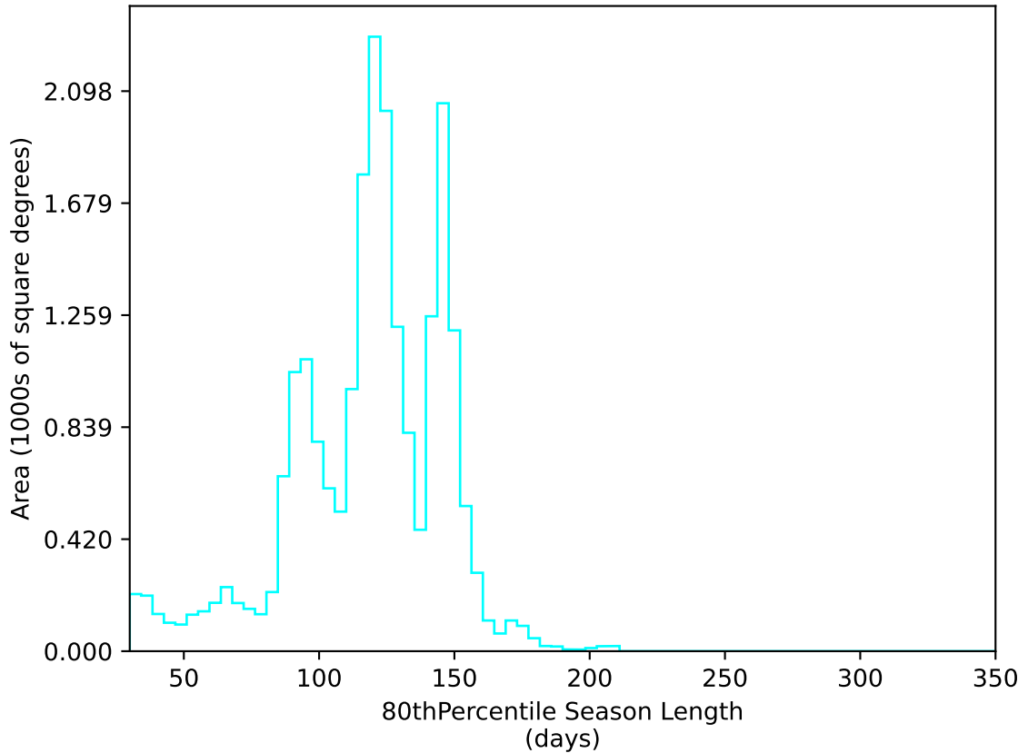
too_elab_r16_d2_griz_v3.4_10yrs All sky u band: 80thPercentile Season Length
