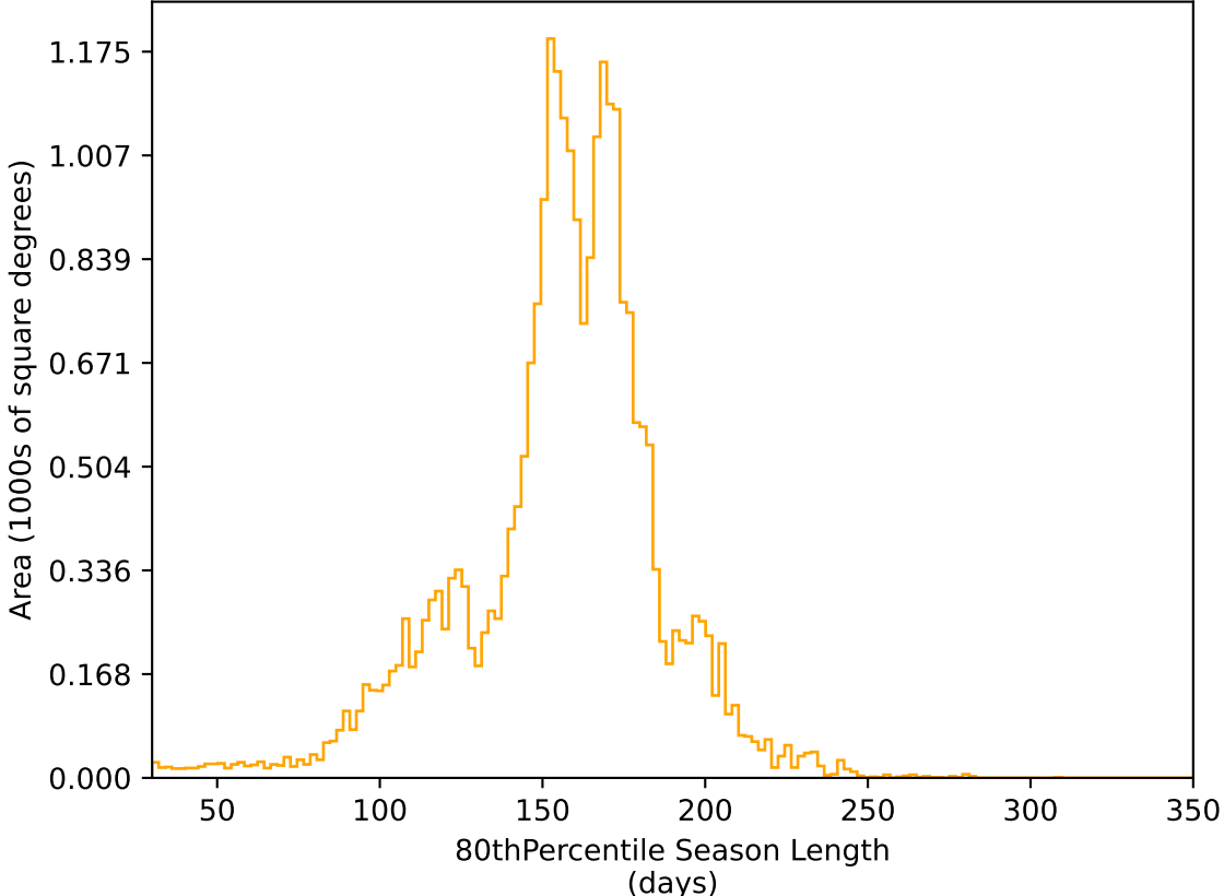
too_elab_r16_d2_griz_v3.4_10yrs All sky r band: 80thPercentile Season Length
