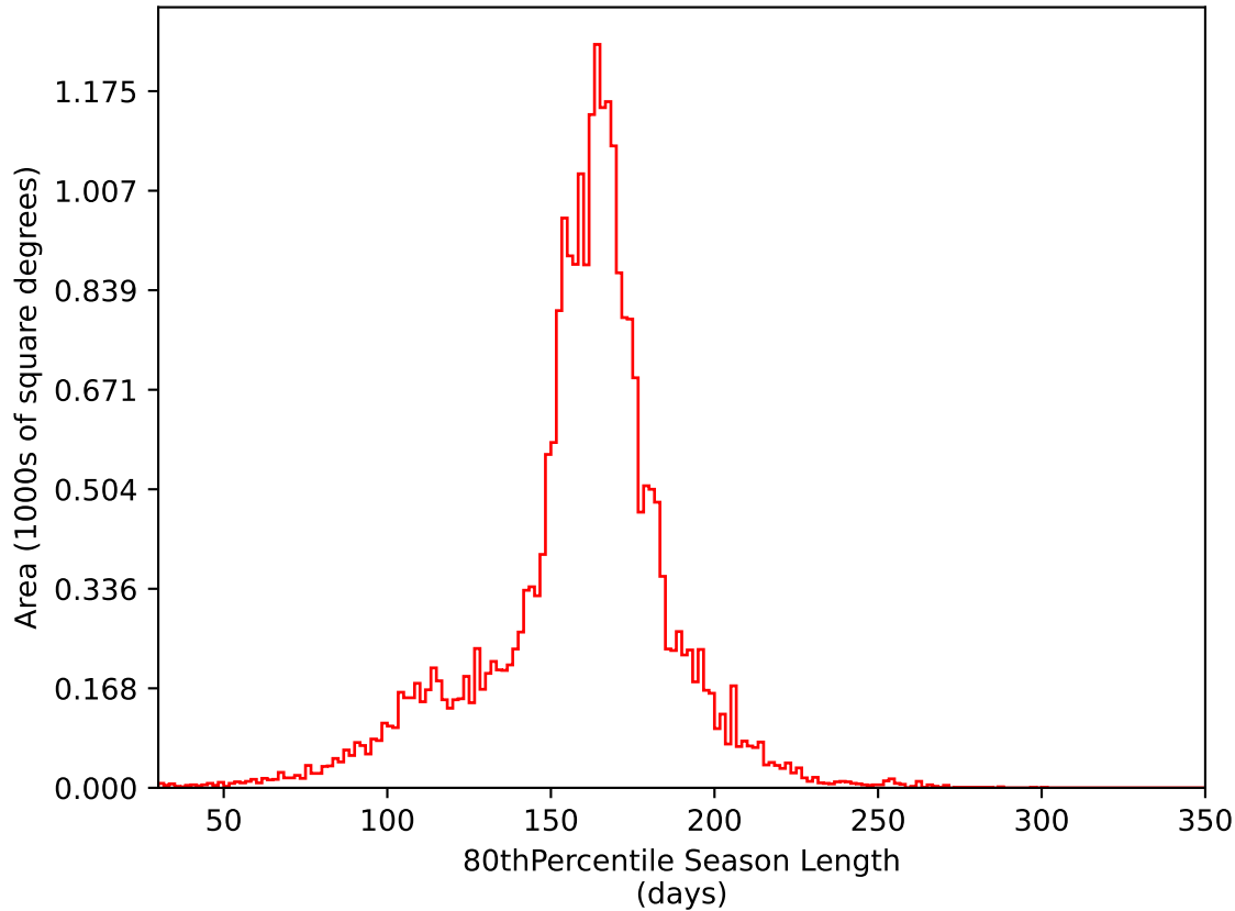
too_elab_r16_d2_griz_v3.4_10yrs All sky i band: 80thPercentile Season Length
