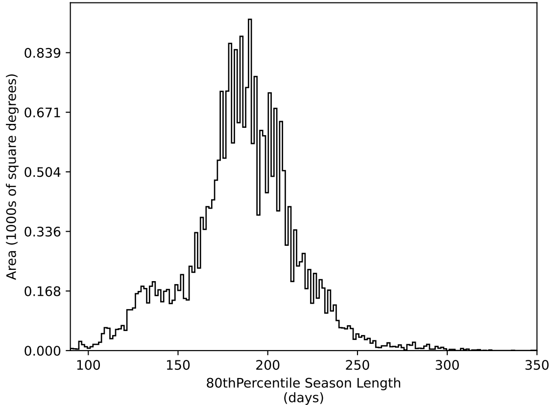
too_elab_r16_d2_griz_v3.4_10yrs All sky all bands: 80thPercentile Season Length
