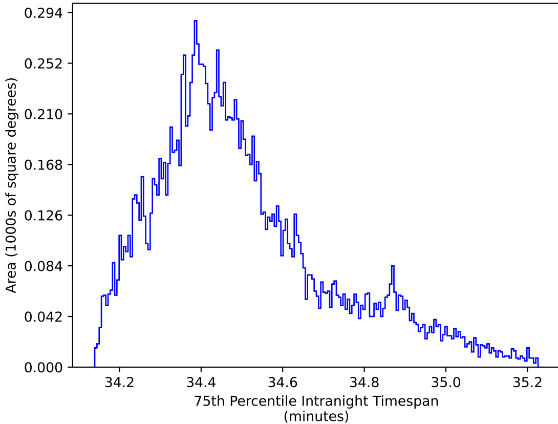
too_elab_r16_d2_griz_v3.4_10yrs WFD zy bands: 75th Percentile Intranight Timespan
