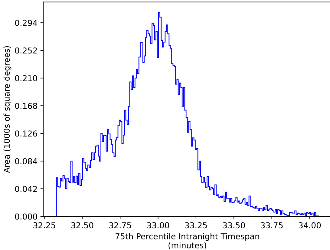
too_elab_r16_d2_griz_v3.4_10yrs WFD y band: 75th Percentile Intranight Timespan
