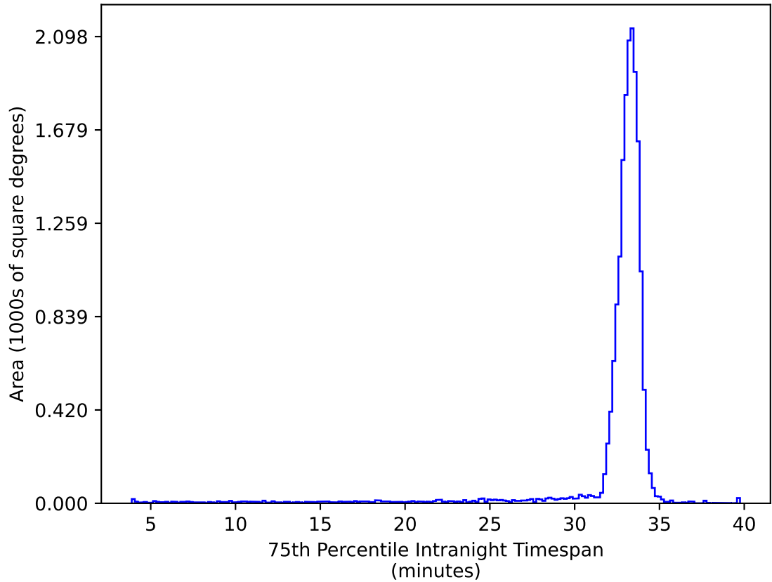
too_elab_r16_d2_griz_v3.4_10yrs WFD ug bands: 75th Percentile Intranight Timespan
