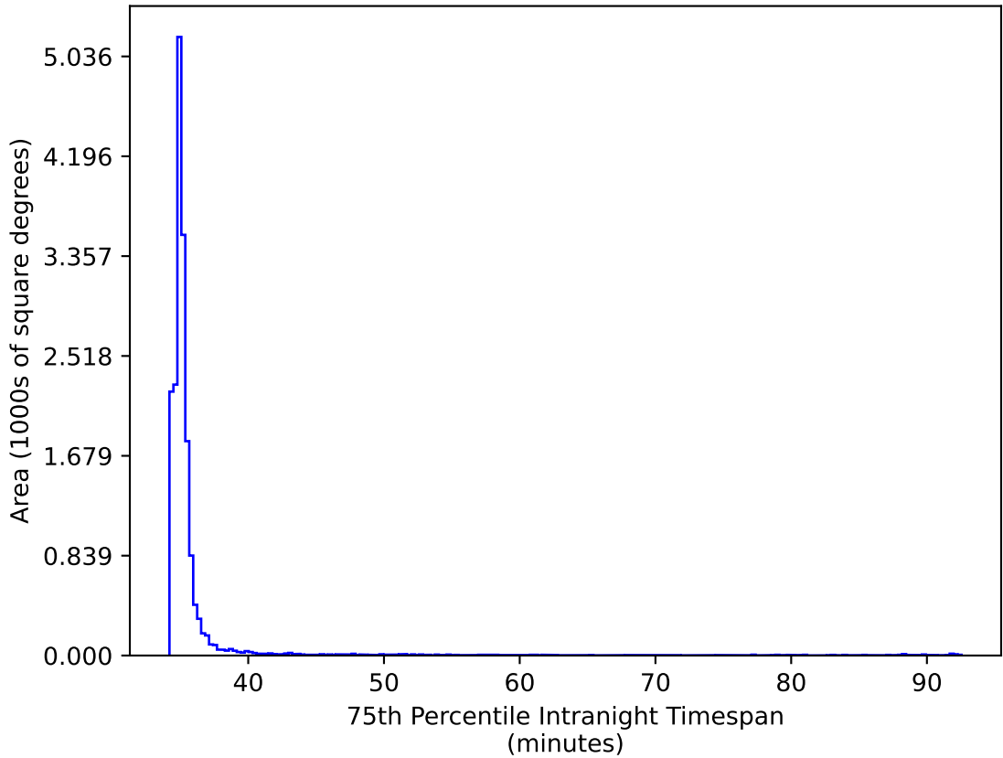
too_elab_r16_d2_griz_v3.4_10yrs WFD ri bands: 75th Percentile Intranight Timespan
