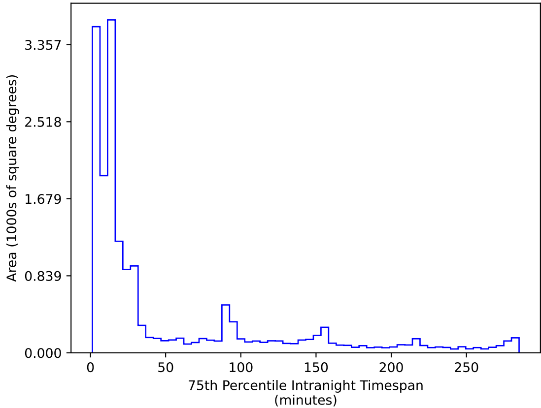
too_elab_r16_d2_griz_v3.4_10yrs WFD r band: 75th Percentile Intranight Timespan
