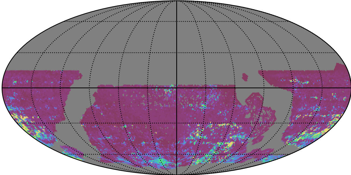
too_elab_r16_d2_griz_v3.4_10yrs WFD i band: 75th Percentile Intranight Timespan
