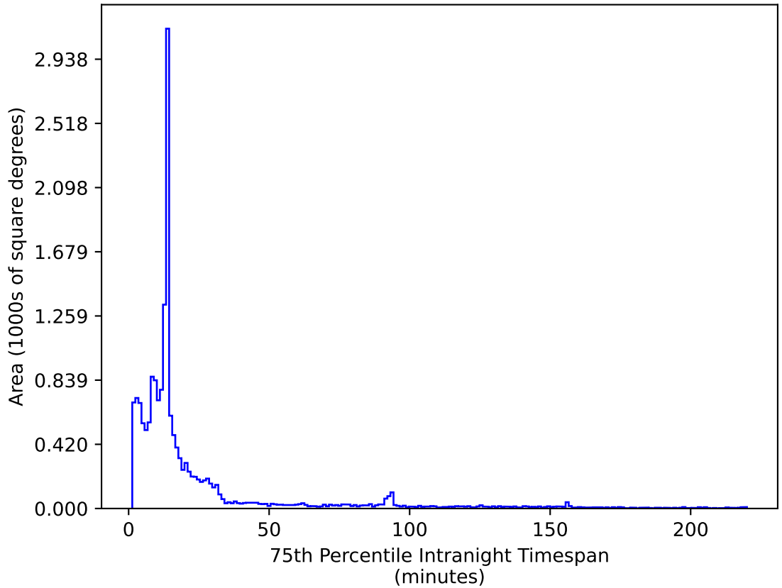
too_elab_r16_d2_griz_v3.4_10yrs WFD i band: 75th Percentile Intranight Timespan
