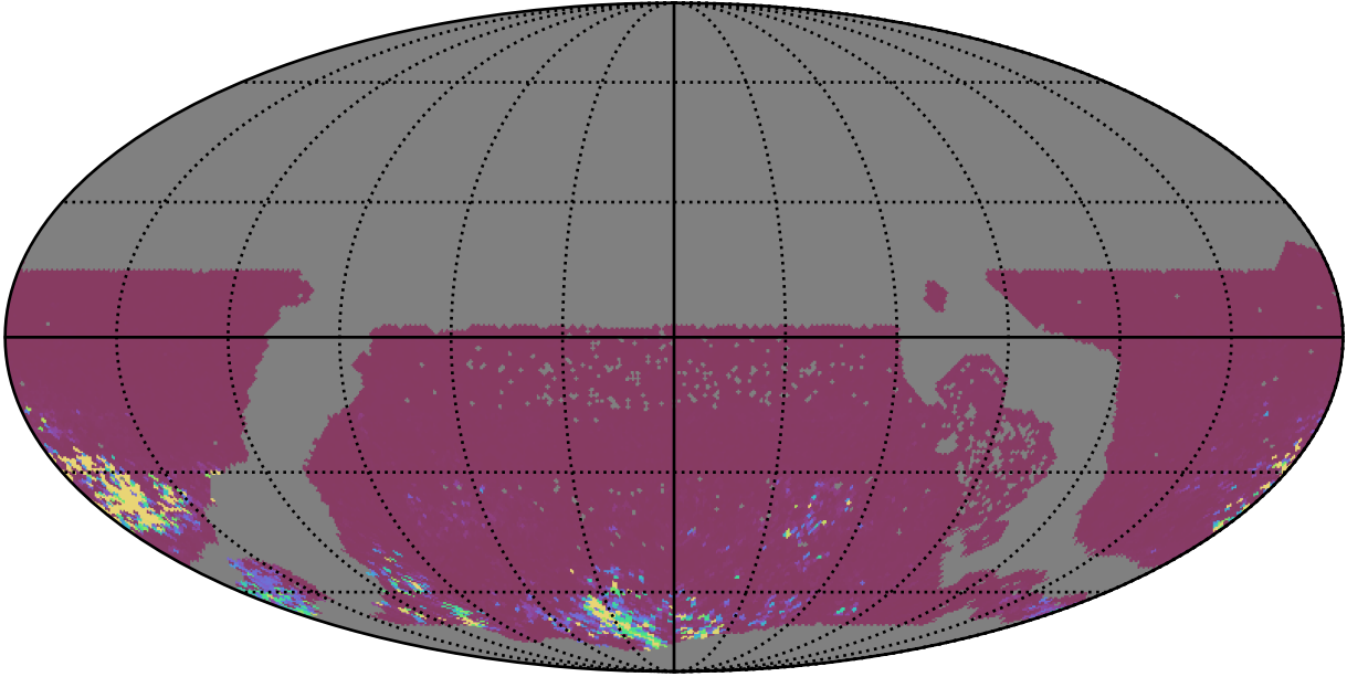
too_elab_r16_d2_griz_v3.4_10yrs WFD gr bands: 75th Percentile Intranight Timespan
