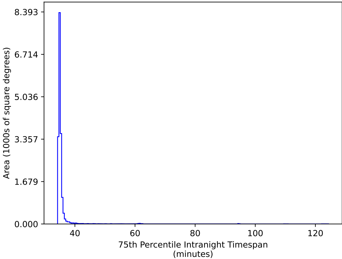
too_elab_r16_d2_griz_v3.4_10yrs WFD gr bands: 75th Percentile Intranight Timespan
