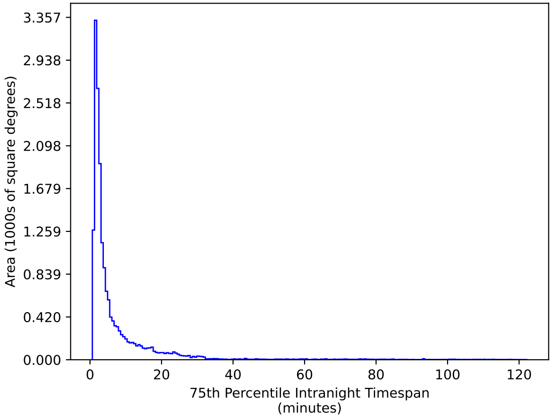
too_elab_r16_d2_griz_v3.4_10yrs WFD g band: 75th Percentile Intranight Timespan
