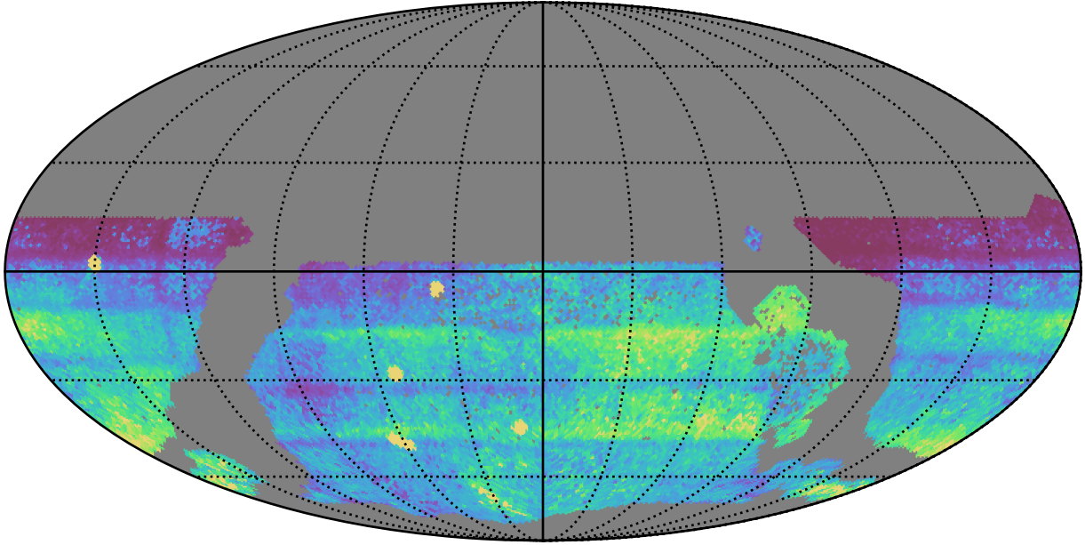
too_elab_r16_d2_griz_v3.4_10yrs WFD all bands: 75th Percentile Intranight Timespan
