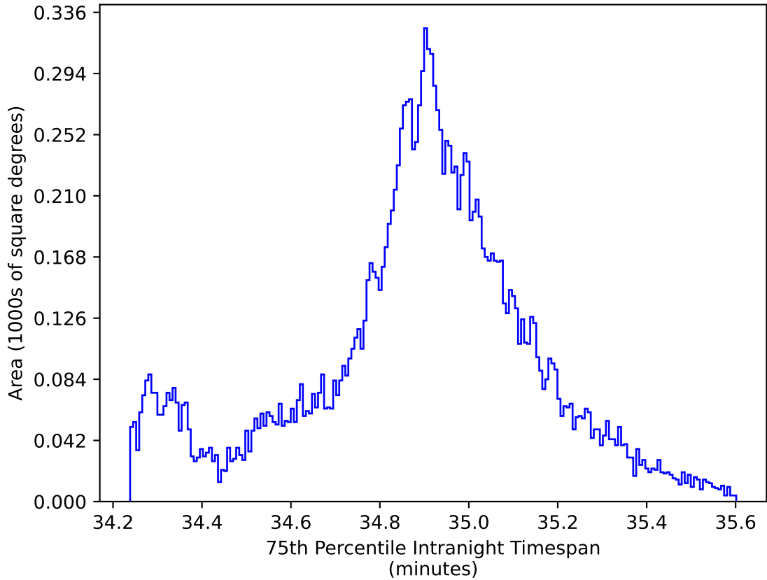
too_elab_r16_d2_griz_v3.4_10yrs WFD all bands: 75th Percentile Intranight Timespan
